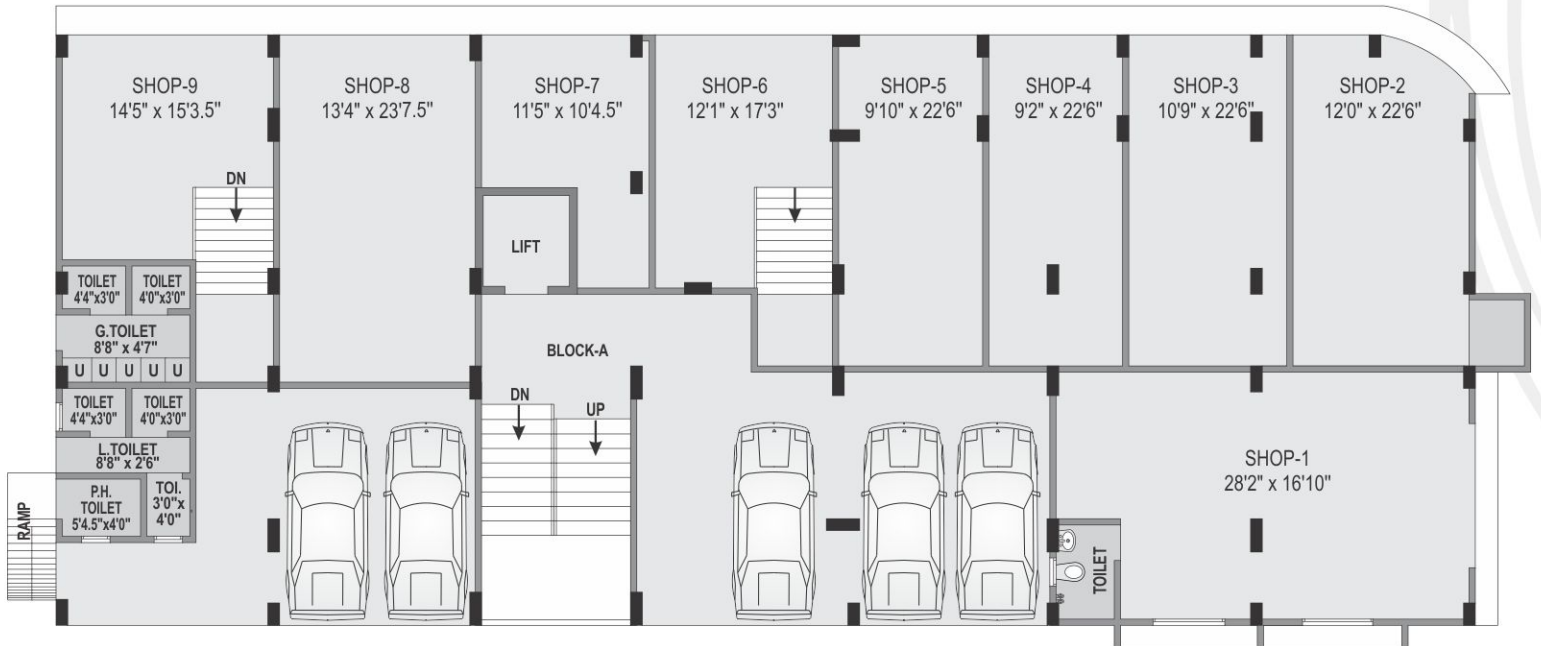
Shop & Parking Plan
