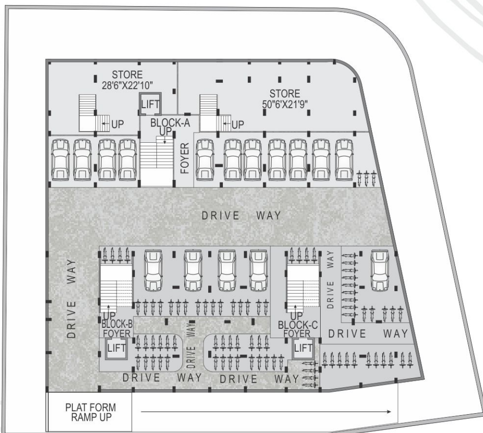
Basement Plan
