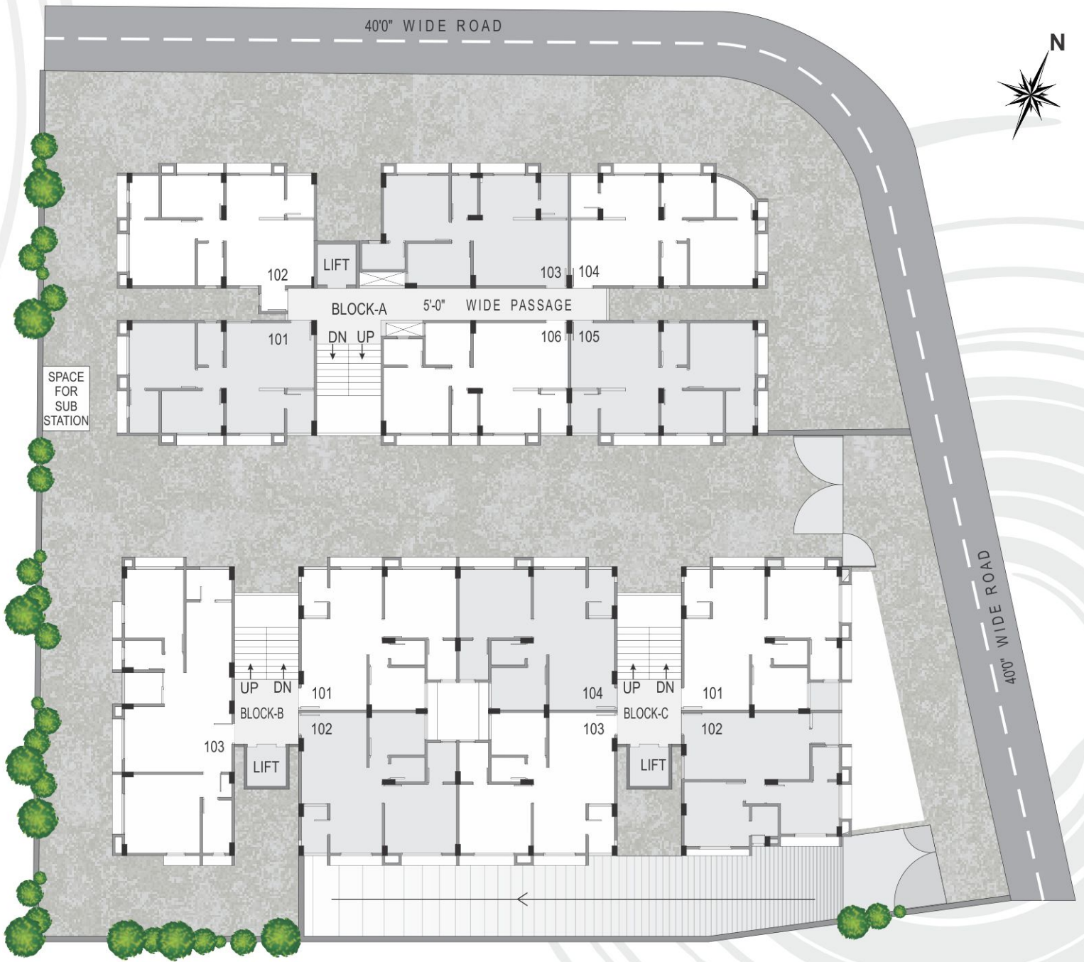
Layout Plan
